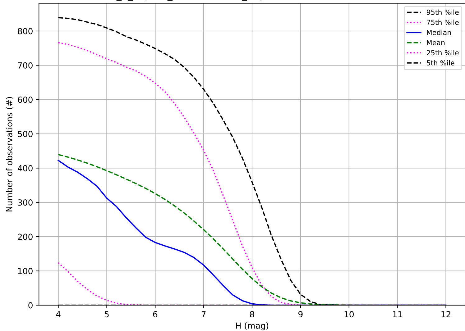
internal_u_expt45_nscale1.5v3.4_10yrs: Number of observations TNO
