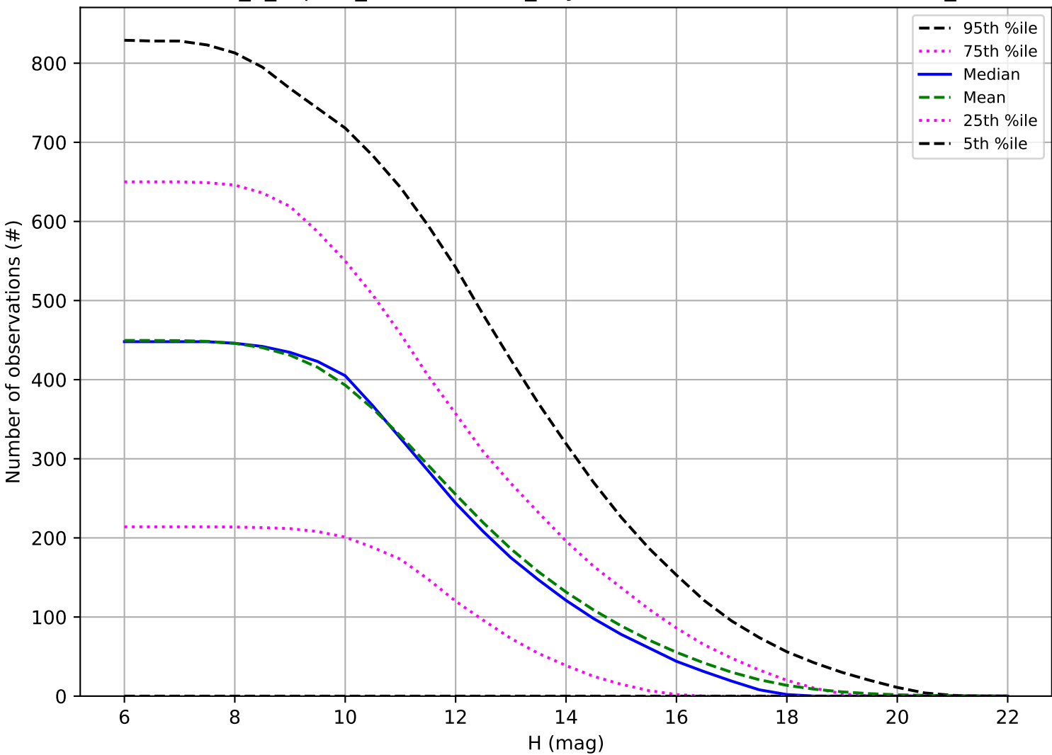
internal_u_expt45_nscale1.5v3.4_10yrs: Number of observations OCC_r5
