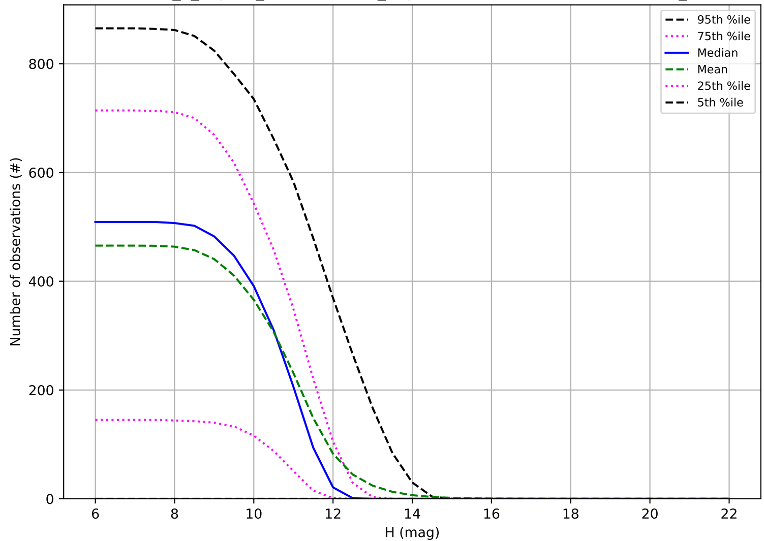
internal_u_expt45_nscale1.5v3.4_10yrs: Number of observations OCC_r20
