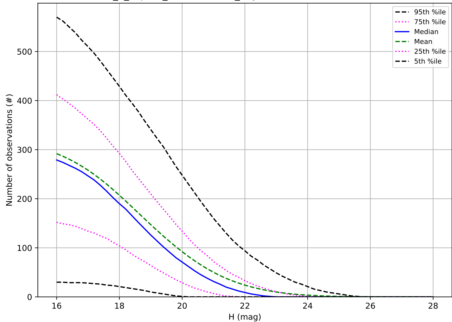
internal_u_expt45_nscale1.5v3.4_10yrs: Number of observations NEO
