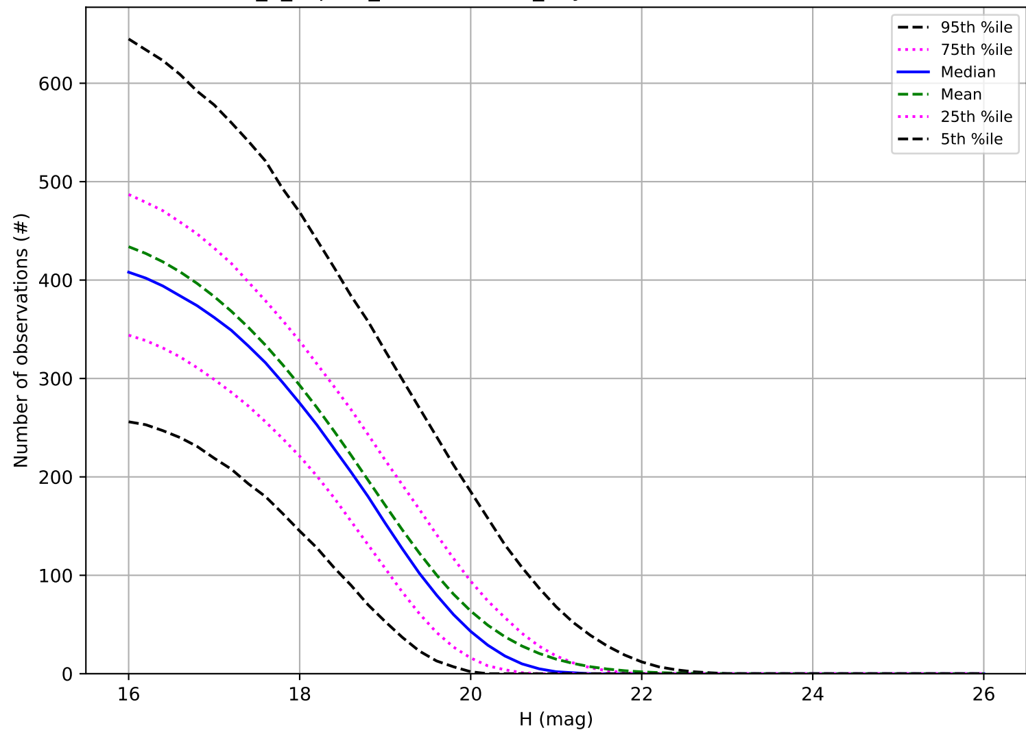
internal_u_expt45_nscale1.5v3.4_10yrs: Number of observations MBA
