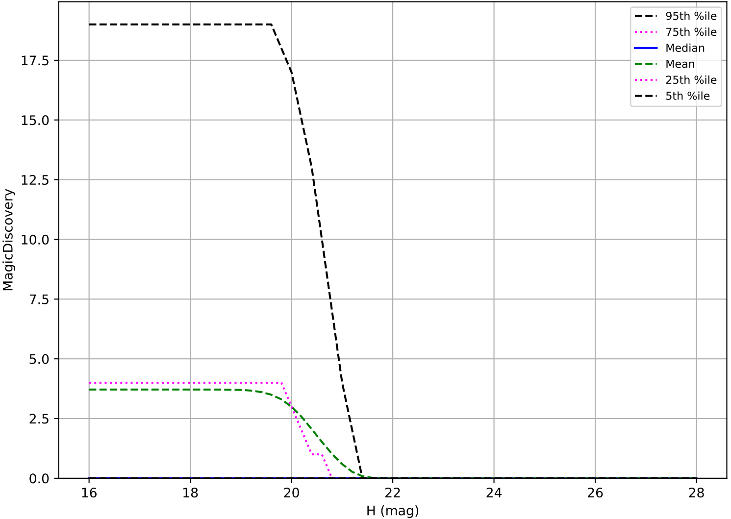
internal_u_expt45_nscale1.5v3.4_10yrs: Vatira 6 detections in 60 nights detection loss
