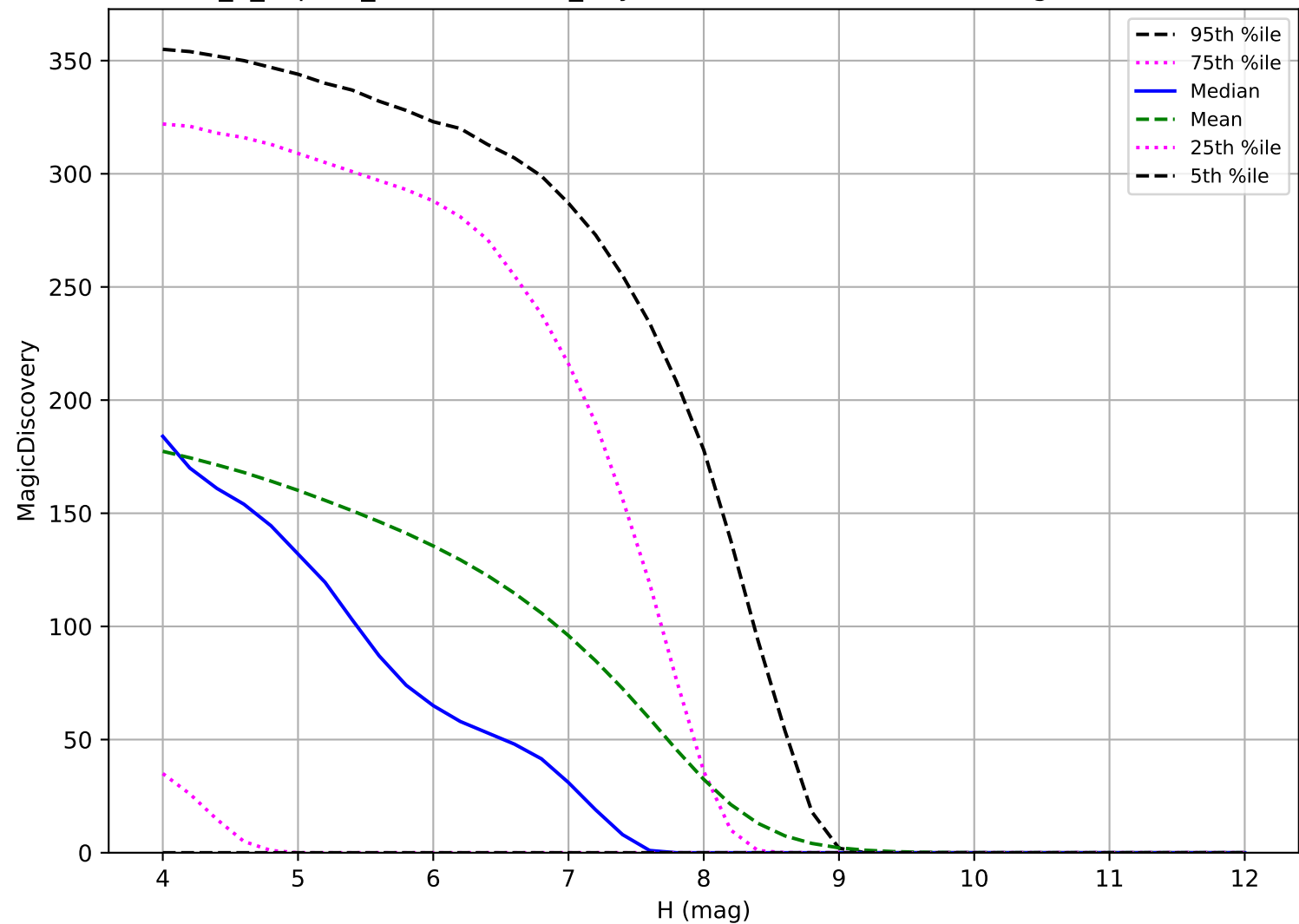
internal_u_expt45_nscale1.5v3.4_10yrs: TNO 6 detections in 60 nights detection loss
