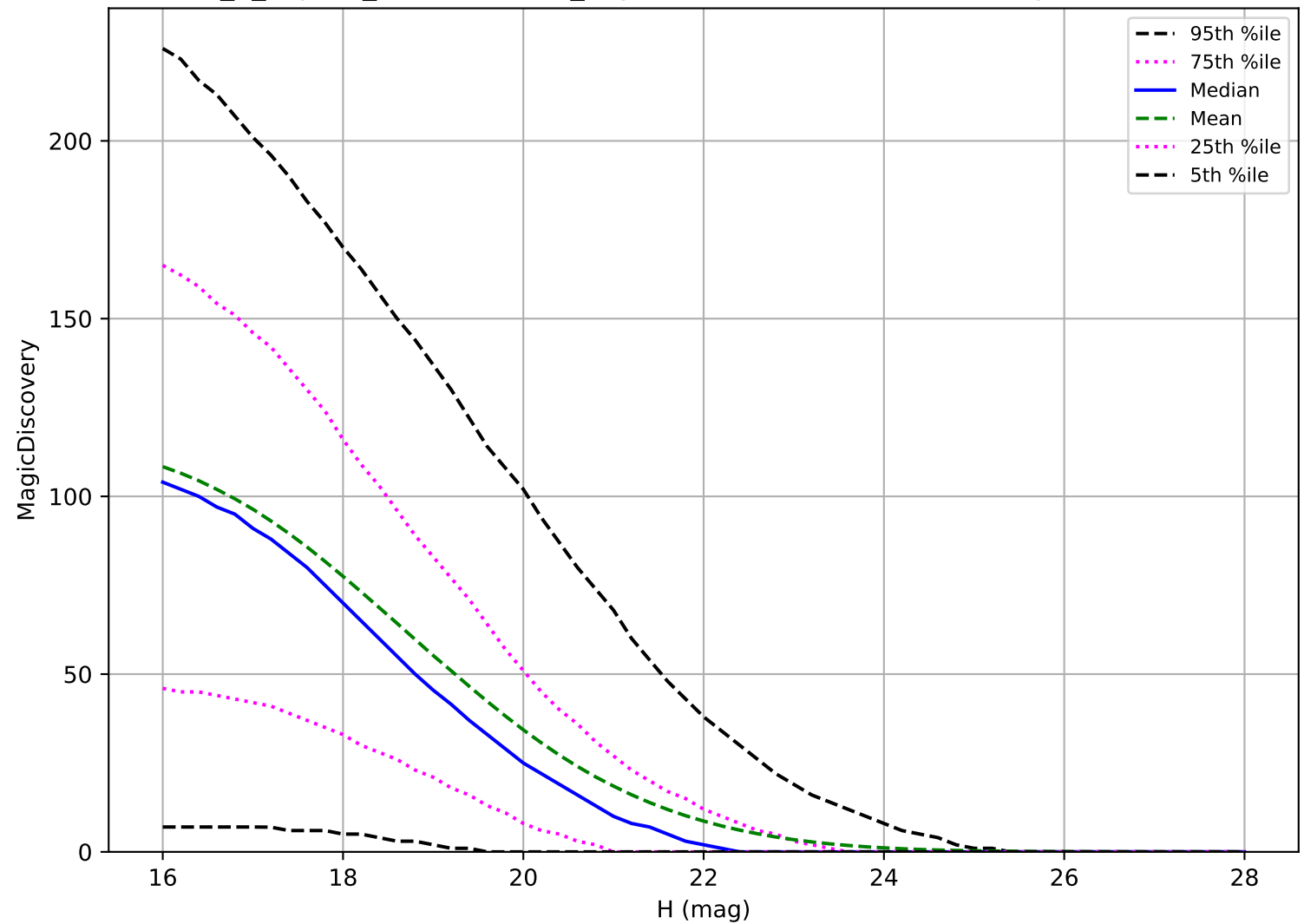
internal_u_expt45_nscale1.5v3.4_10yrs: PHA 6 detections in 60 nights detection loss
