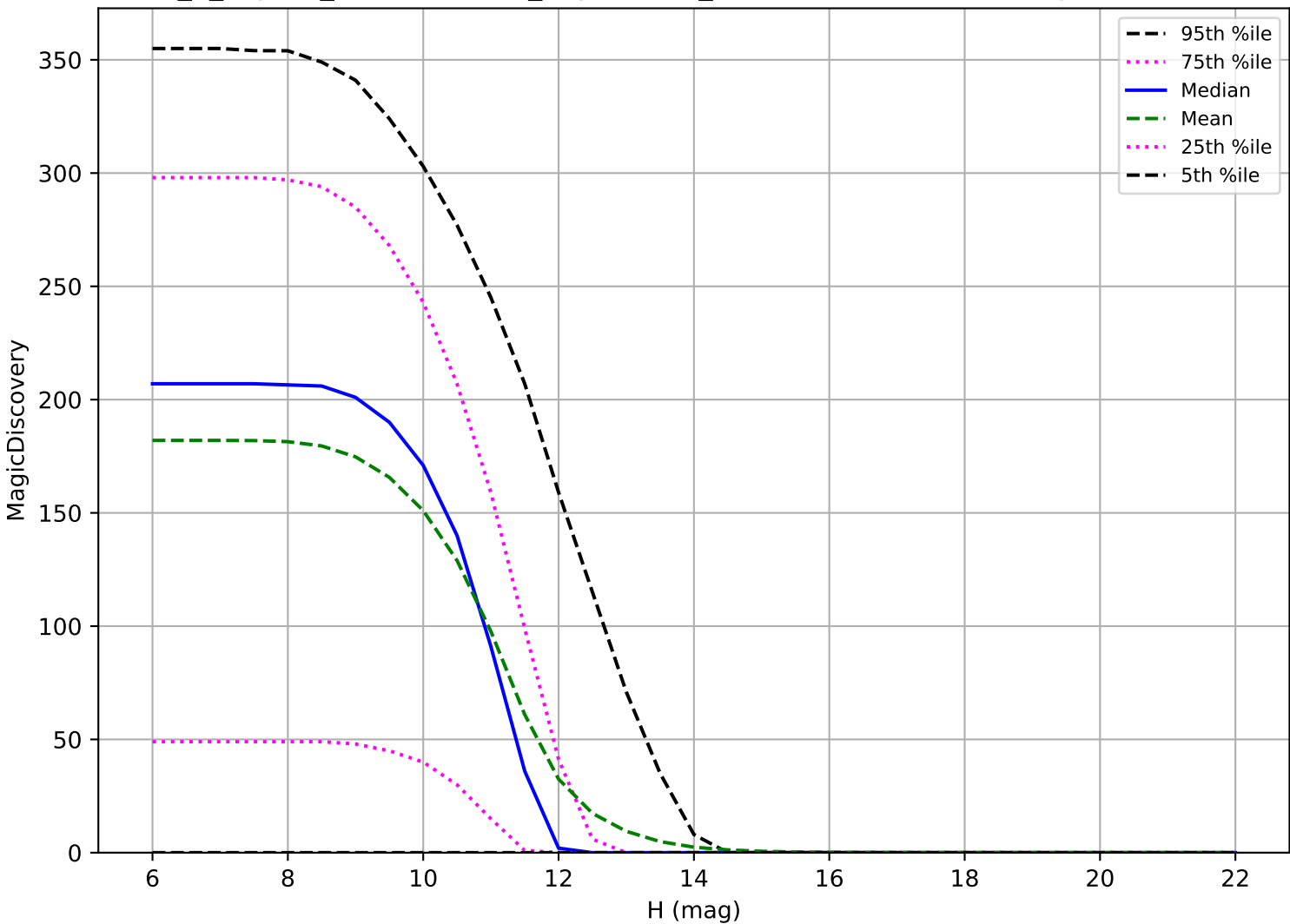
internal_u_expt45_nscale1.5v3.4_10yrs: OCC_r20 6 detections in 60 nights detection loss
