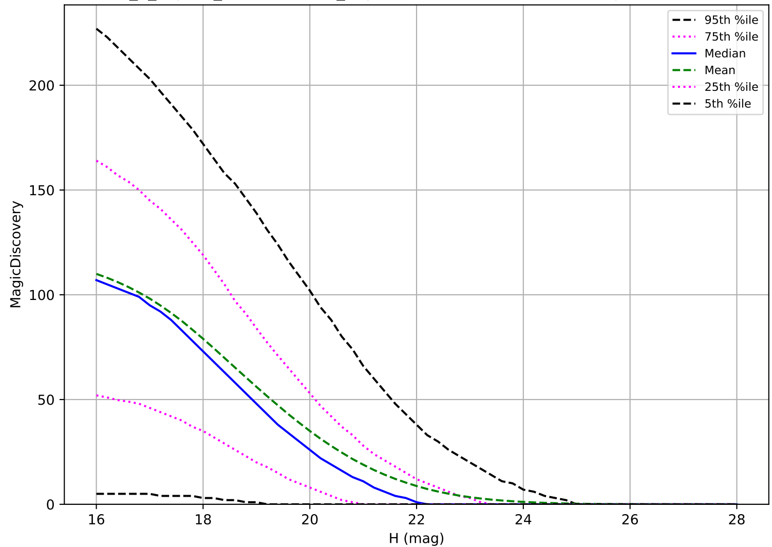
internal_u_expt45_nscale1.5v3.4_10yrs: NEO 6 detections in 60 nights detection loss
