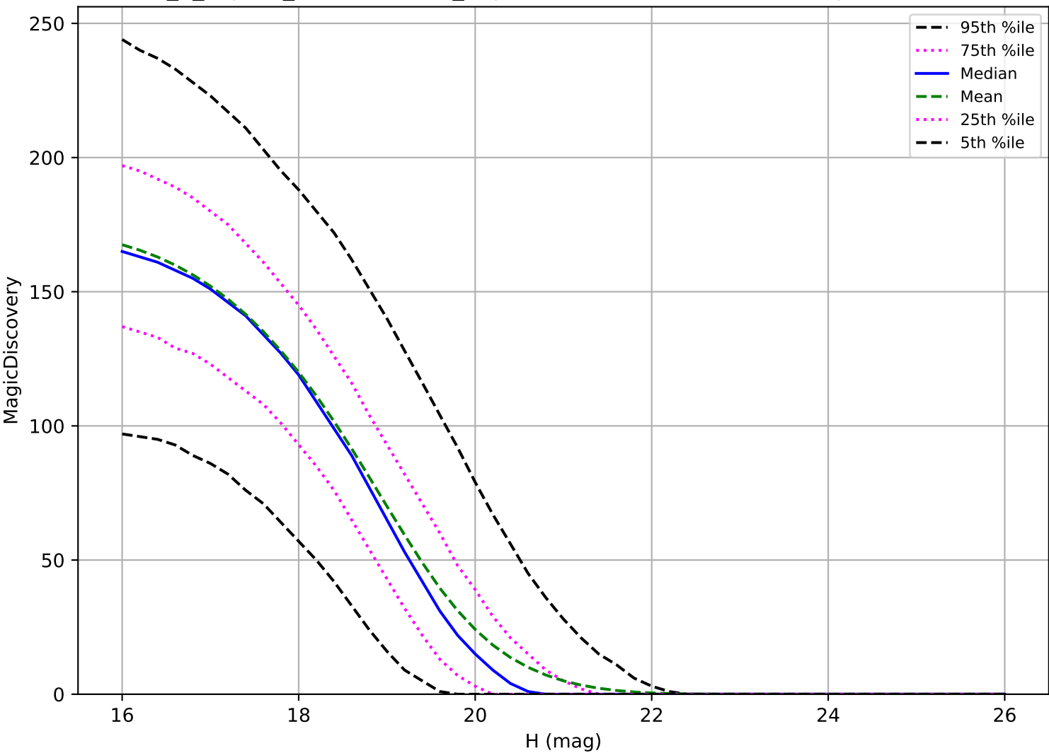
internal_u_expt45_nscale1.5v3.4_10yrs: MBA 6 detections in 60 nights detection loss
