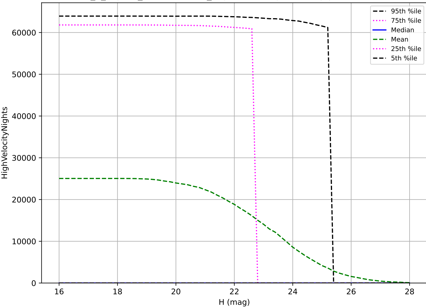
internal_u_expt45_nscale1.5v3.4_10yrs: PHA High velocity pair detection loss
