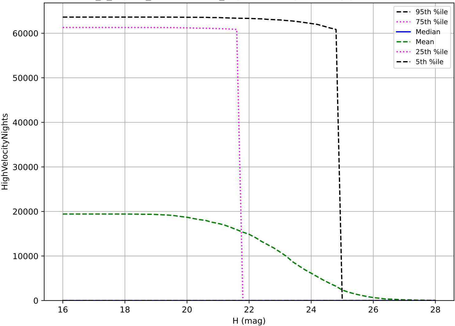
internal_u_expt45_nscale1.5v3.4_10yrs: NEO High velocity pair detection loss
