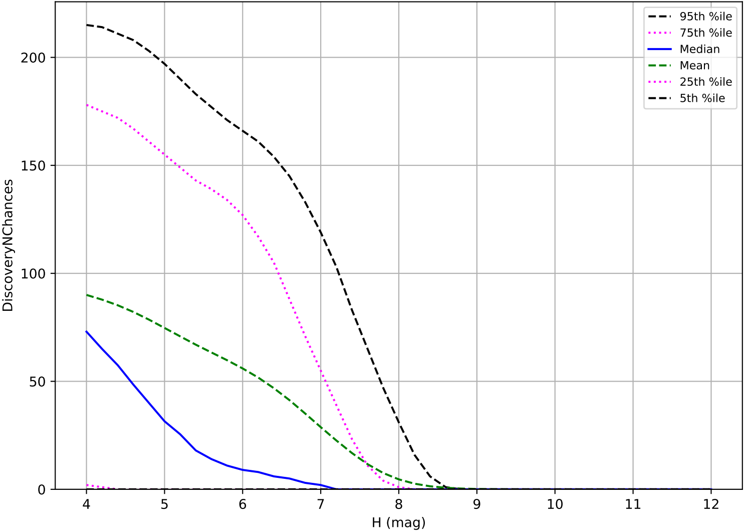
internal_u_expt45_nscale1.5v3.4_10yrs: TNO 3 pairs in 15 nights detection loss
