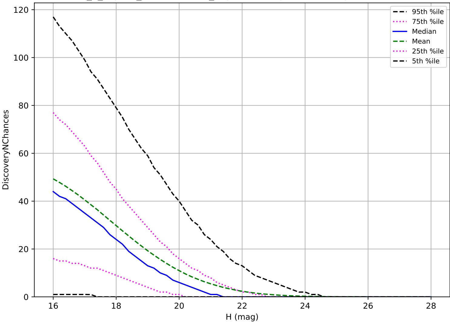
internal_u_expt45_nscale1.5v3.4_10yrs: PHA 3 pairs in 15 nights detection loss
