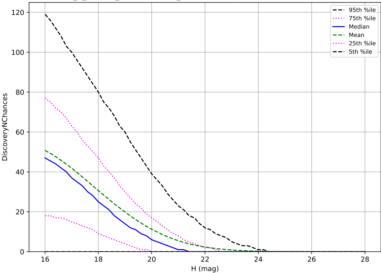
internal_u_expt45_nscale1.5v3.4_10yrs: NEO 3 pairs in 15 nights detection loss
