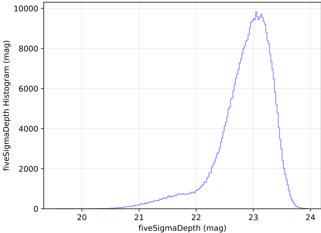
internal_u_expt45_nscale1.5v3.4_10yrs z: fiveSigmaDepth Histogram
