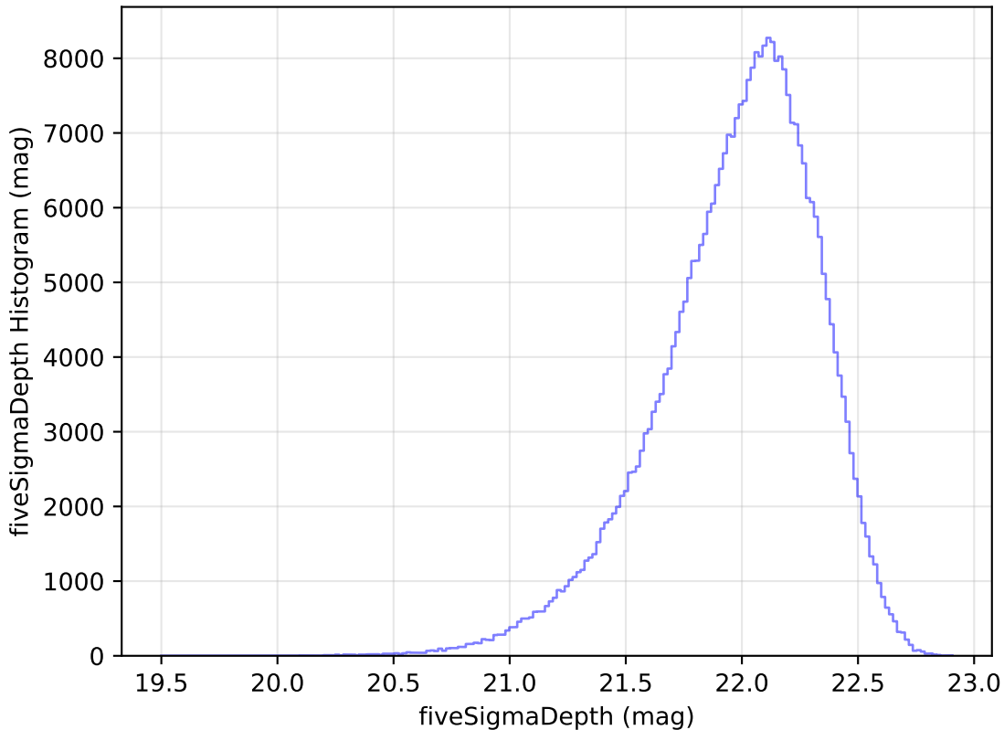
internal_u_expt45_nscale1.5v3.4_10yrs y: fiveSigmaDepth Histogram
