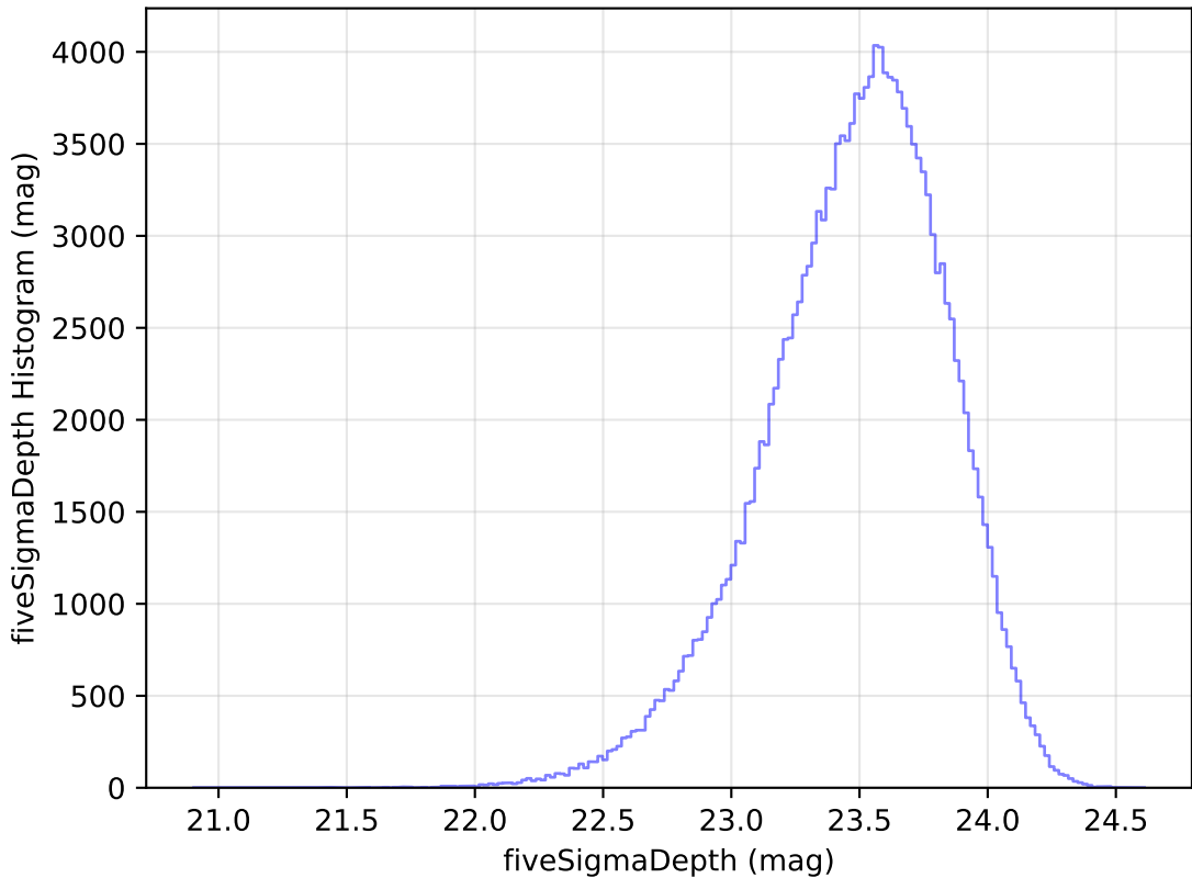
internal_u_expt45_nscale1.5v3.4_10yrs u: fiveSigmaDepth Histogram
