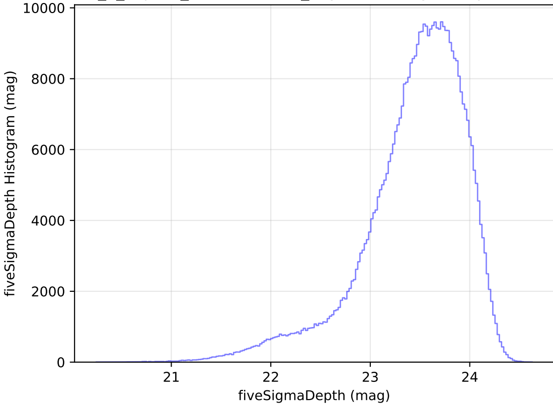
internal_u_expt45_nscale1.5v3.4_10yrs i: fiveSigmaDepth Histogram
