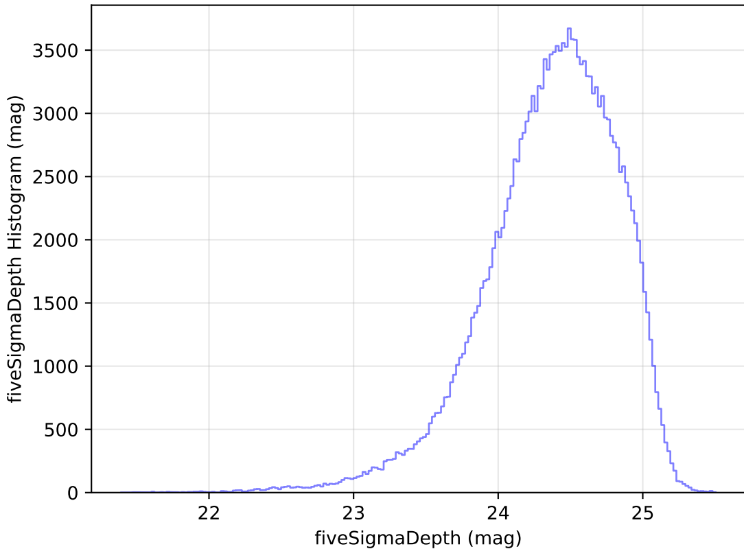
internal_u_expt45_nscale1.5v3.4_10yrs g: fiveSigmaDepth Histogram
