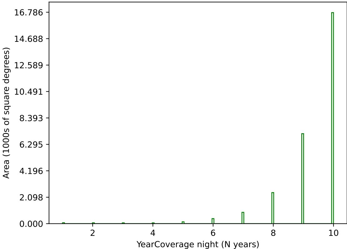
internal_u_expt45_nscale1.5v3.4_10yrs g band: YearCoverage night
