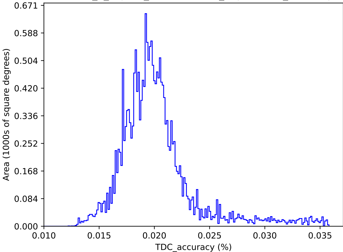
internal_u_expt45_nscale1.5v3.4_10yrs : TDC_accuracy
