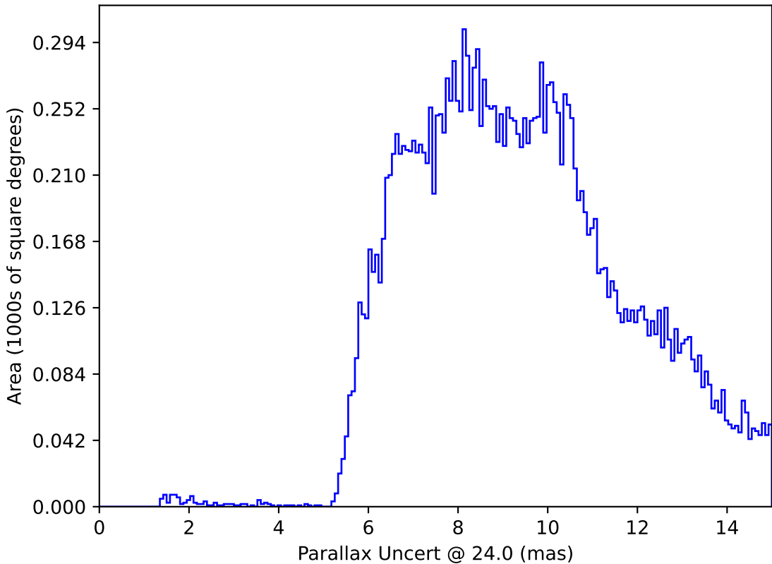
internal_u_expt45_nscale1.5v3.4_10yrs : Parallax Uncert @ 24.0
