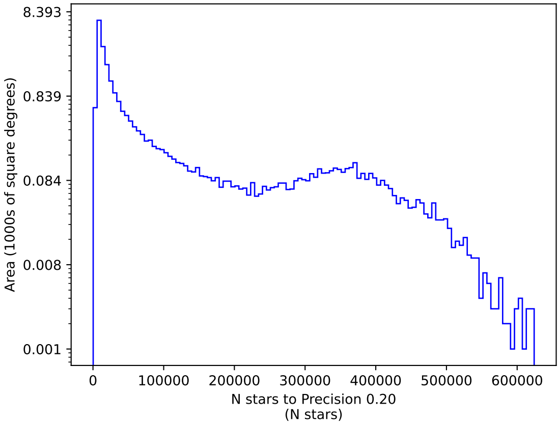
internal_u_expt45_nscale1.5v3.4_10yrs y: N stars to Precision 0.20
