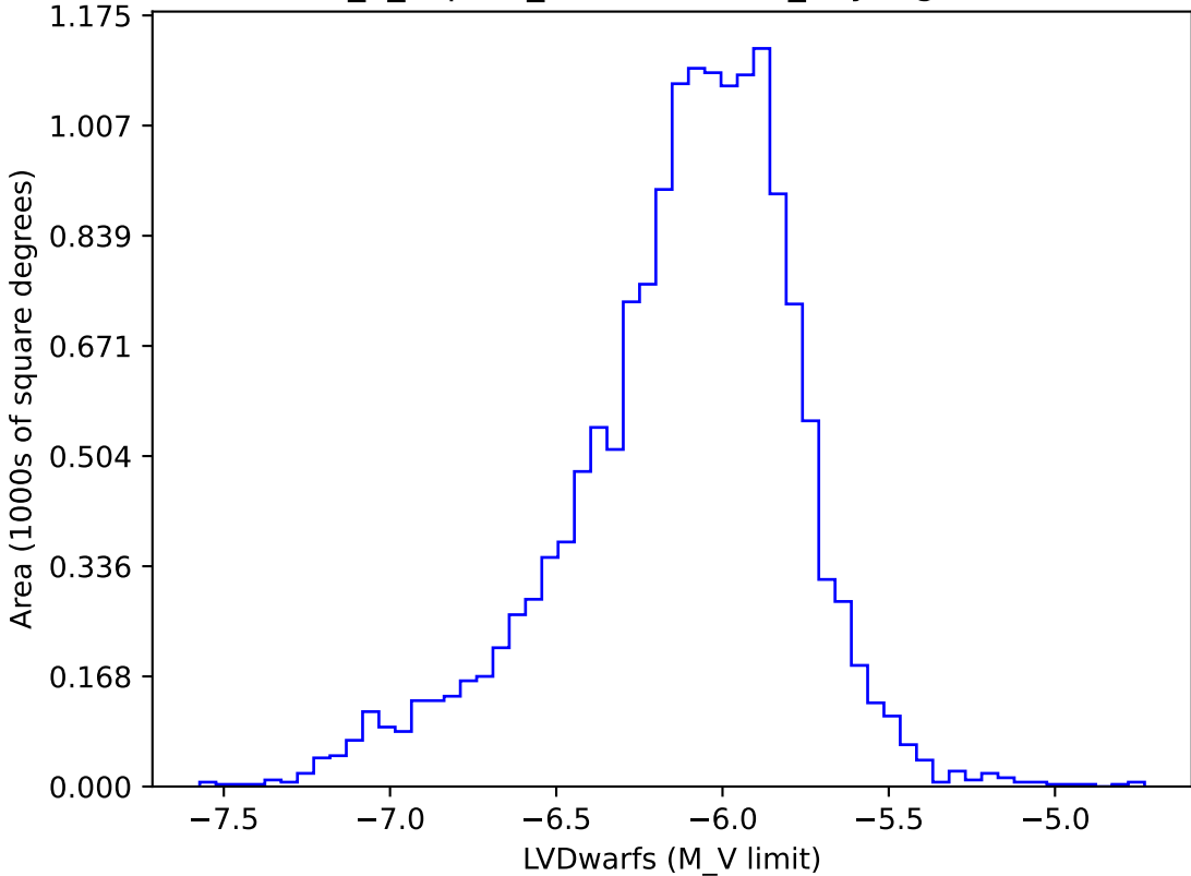
internal_u_expt45_nscale1.5v3.4_10yrs gi: LVDwarfs
