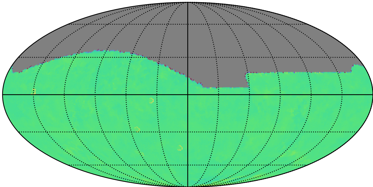
internal_u_expt45_nscale1.5v3.4_10yrs i: Kuiper rotTelPos
