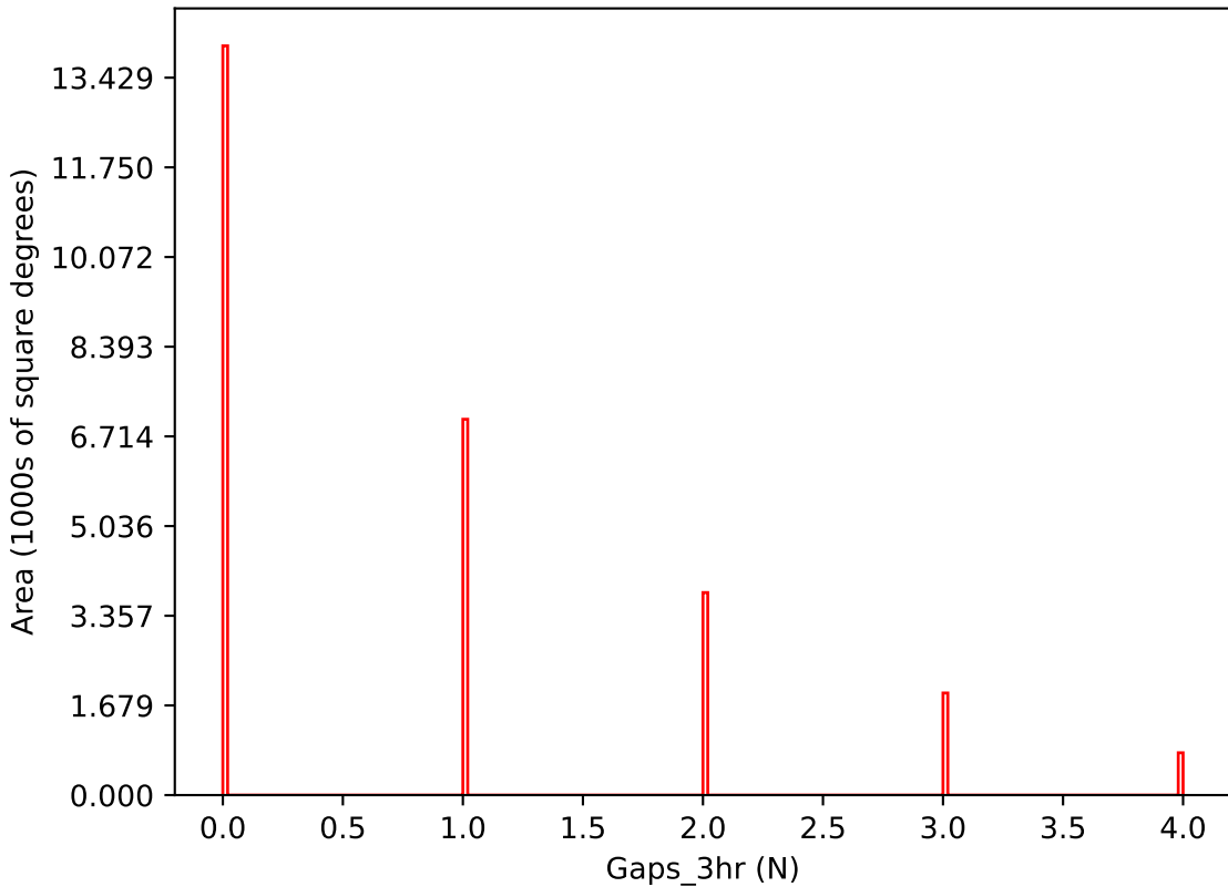
internal_u_expt45_nscale1.5v3.4_10yrs i band: Gaps_3hr
