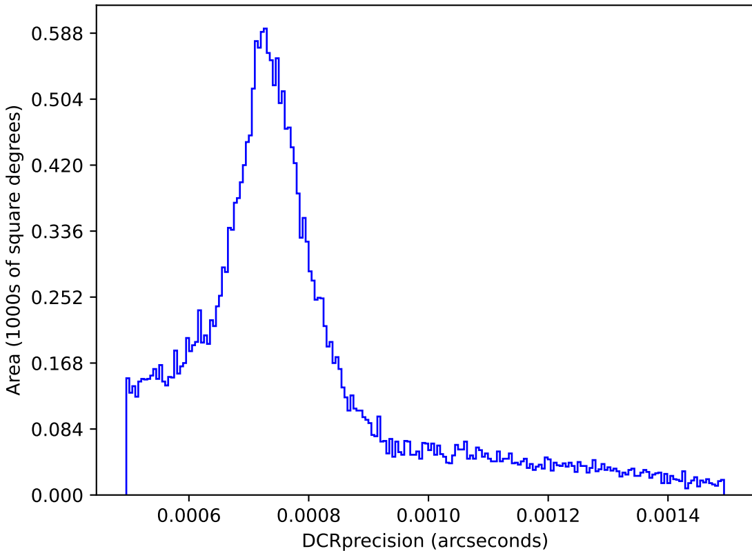
internal_u_expt45_nscale1.5v3.4_10yrs : DCRprecision
