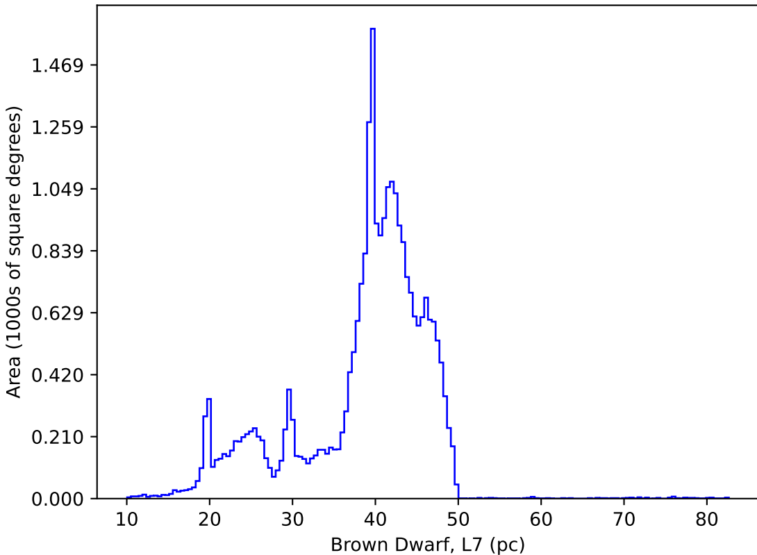
internal_u_expt45_nscale1.5v3.4_10yrs : Brown Dwarf, L7
