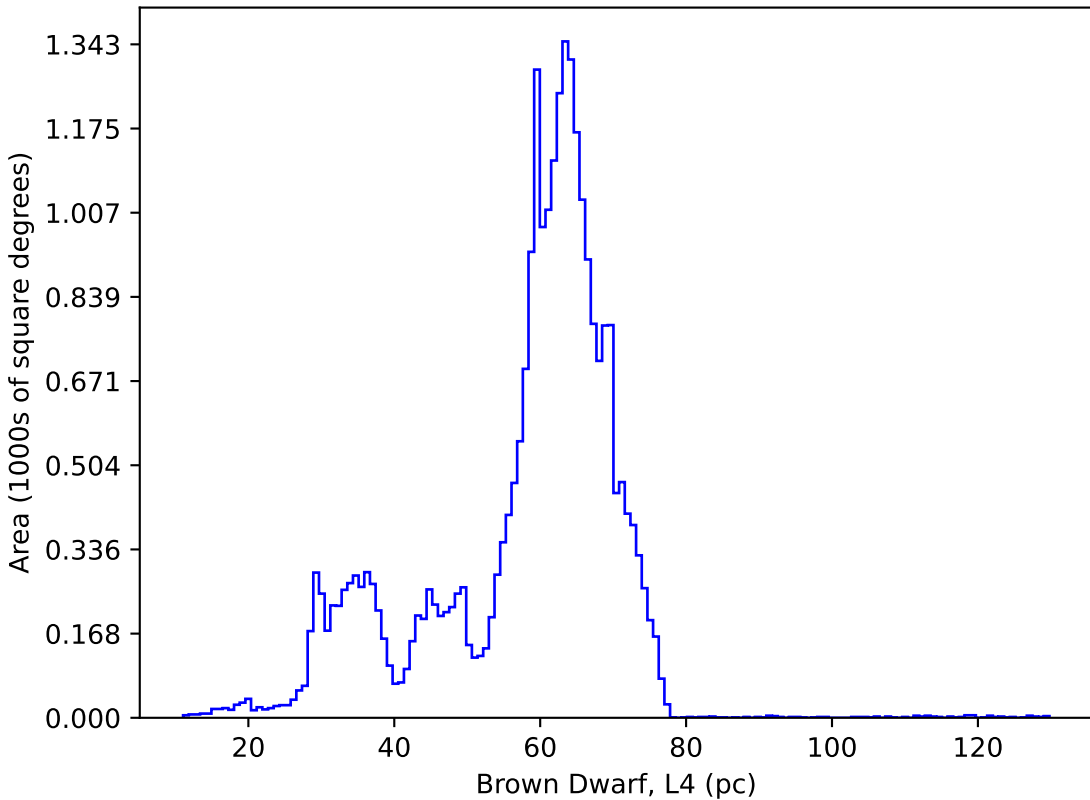
internal_u_expt45_nscale1.5v3.4_10yrs : Brown Dwarf, L4
