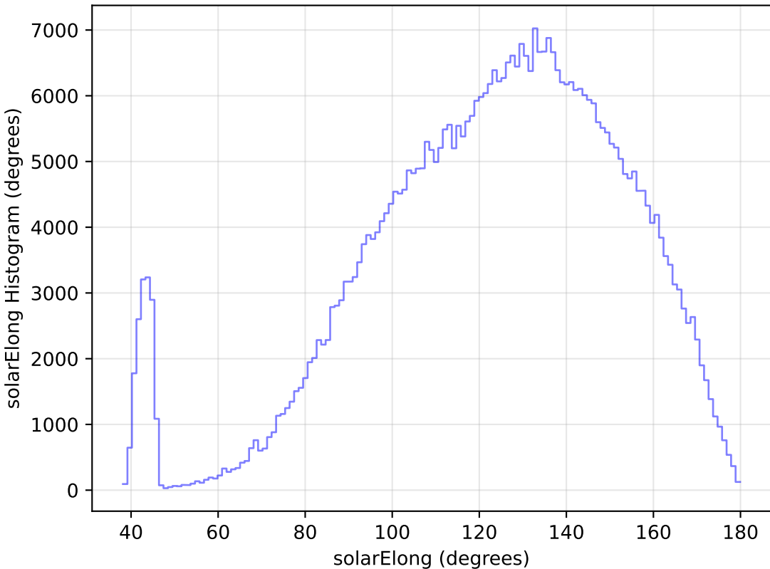
internal_u_expt45_nscale1.5v3.4_10yrs WFD r band: solarElong Histogram
