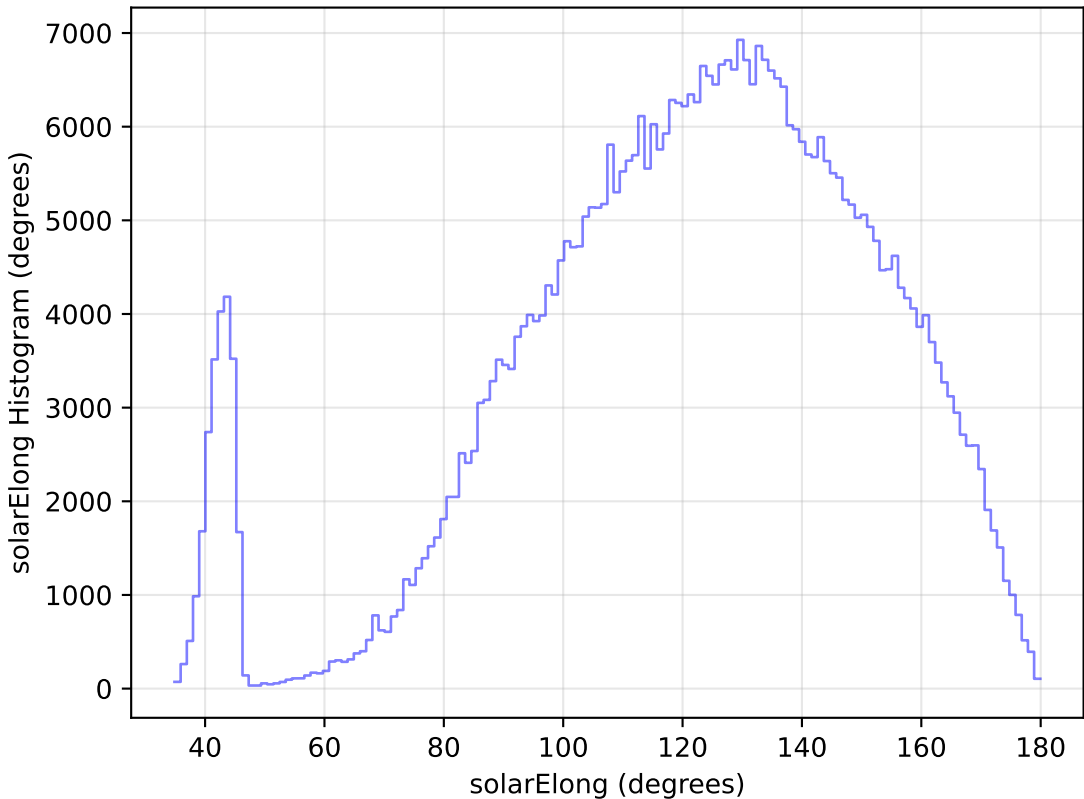
internal_u_expt45_nscale1.5v3.4_10yrs WFD i band: solarElong Histogram
