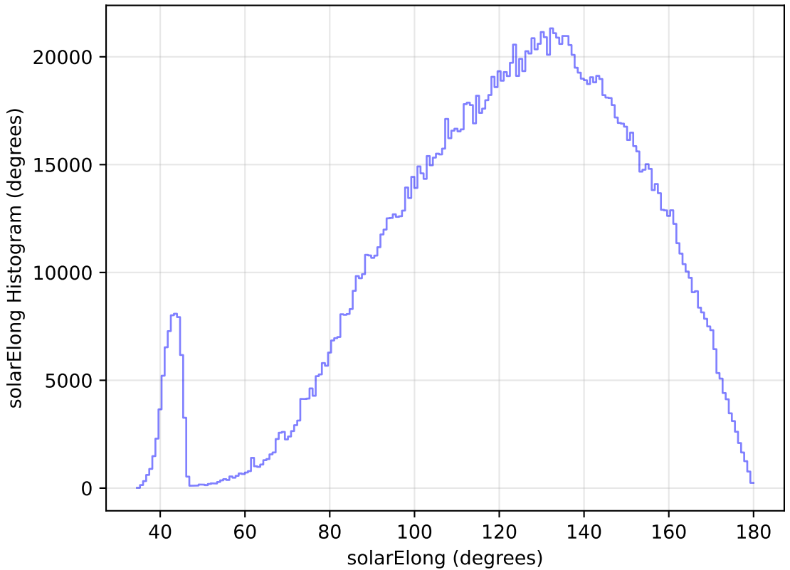
internal_u_expt45_nscale1.5v3.4_10yrs WFD all bands: solarElong Histogram
