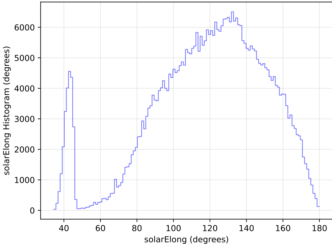
internal_u_expt45_nscale1.5v3.4_10yrs All sky z band: solarElong Histogram
