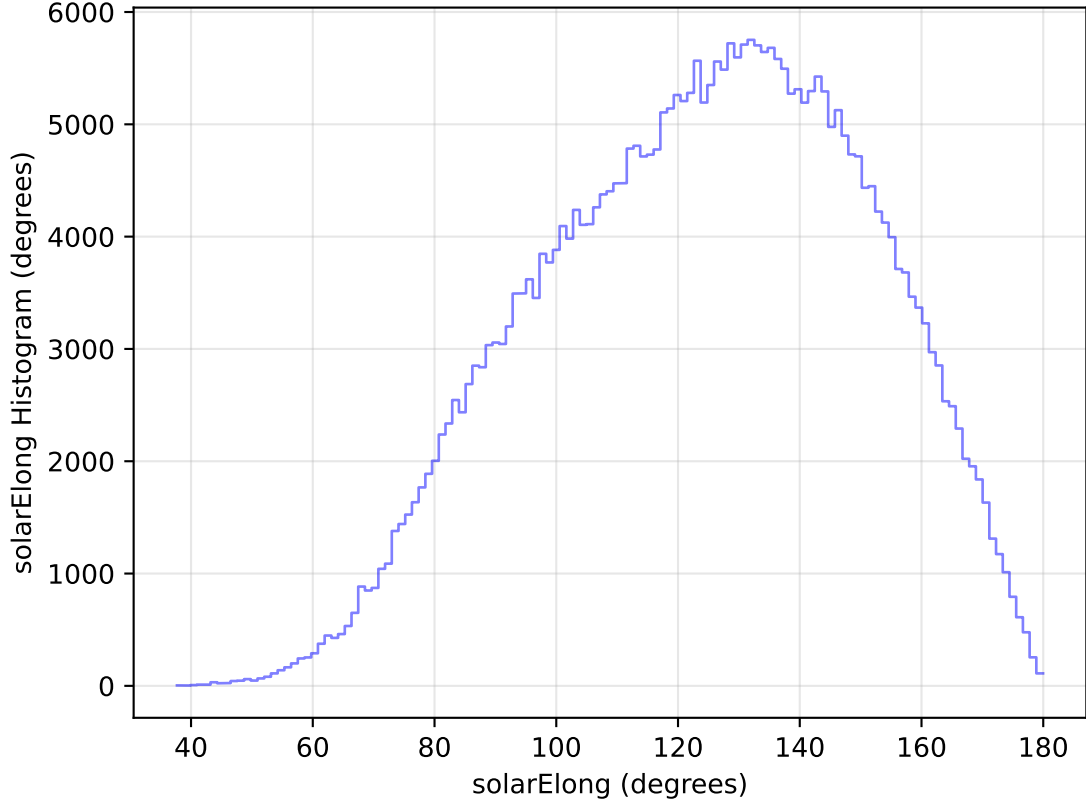
internal_u_expt45_nscale1.5v3.4_10yrs All sky y band: solarElong Histogram
