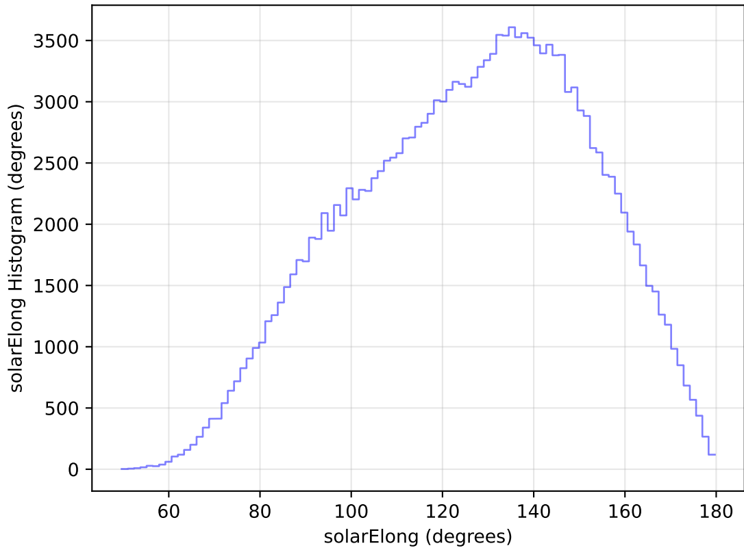
internal_u_expt45_nscale1.5v3.4_10yrs All sky u band: solarElong Histogram
