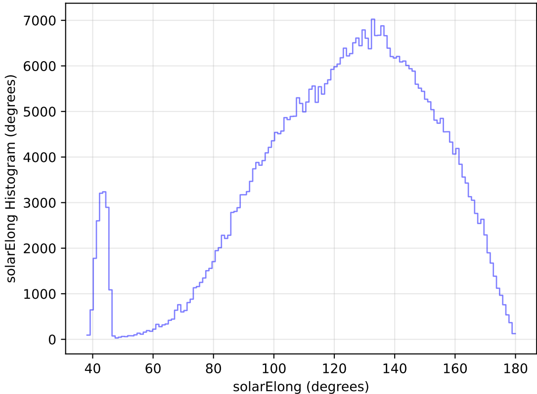
internal_u_expt45_nscale1.5v3.4_10yrs All sky r band: solarElong Histogram
