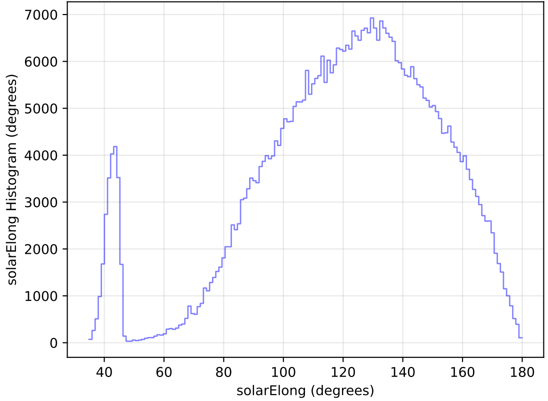
internal_u_expt45_nscale1.5v3.4_10yrs All sky i band: solarElong Histogram
