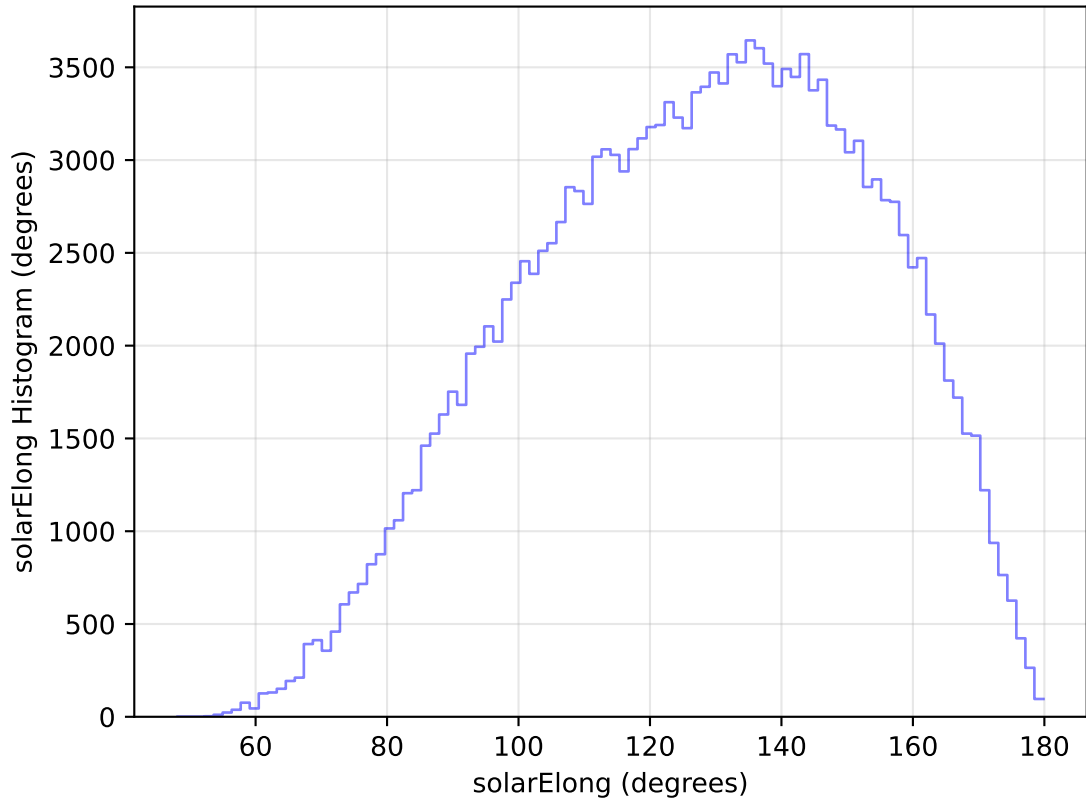
internal_u_expt45_nscale1.5v3.4_10yrs All sky g band: solarElong Histogram
