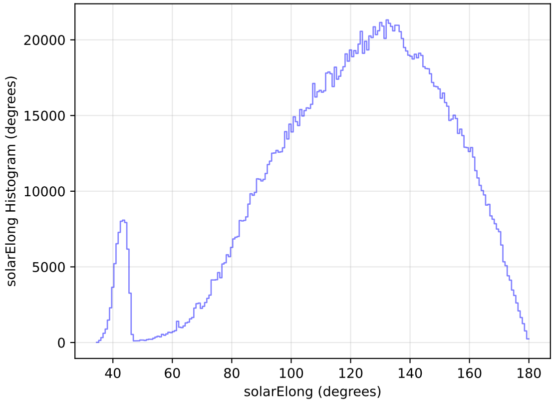
internal_u_expt45_nscale1.5v3.4_10yrs All sky all bands: solarElong Histogram
