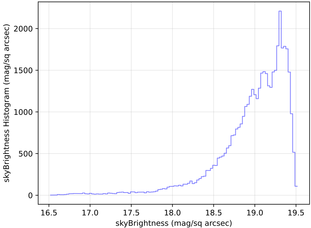
internal_u_expt45_nscale1.5v3.4_10yrs Yr 1 z band: skyBrightness Histogram
