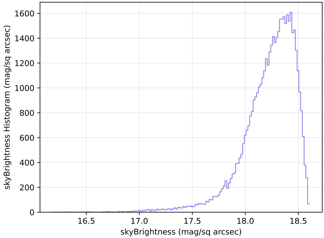
internal_u_expt45_nscale1.5v3.4_10yrs Yr 1 y band: skyBrightness Histogram
