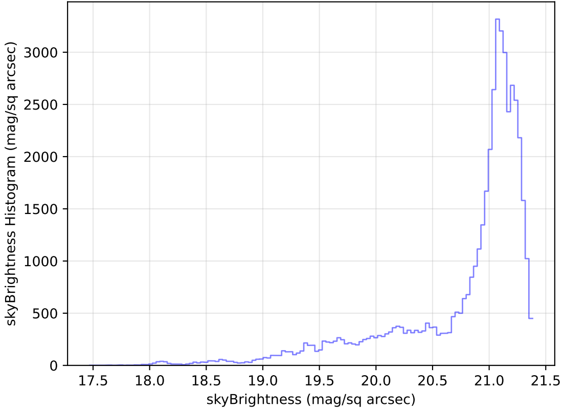
internal_u_expt45_nscale1.5v3.4_10yrs Yr 1 r band: skyBrightness Histogram
