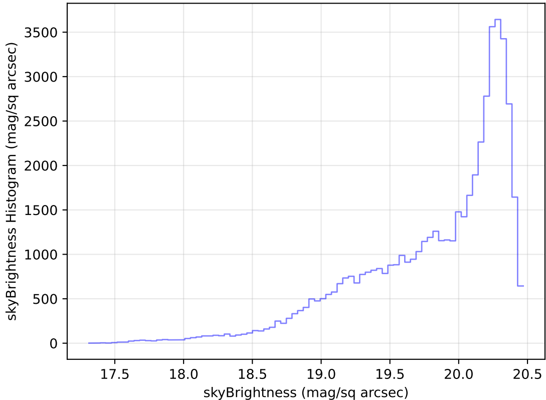
internal_u_expt45_nscale1.5v3.4_10yrs Yr 1 i band: skyBrightness Histogram
