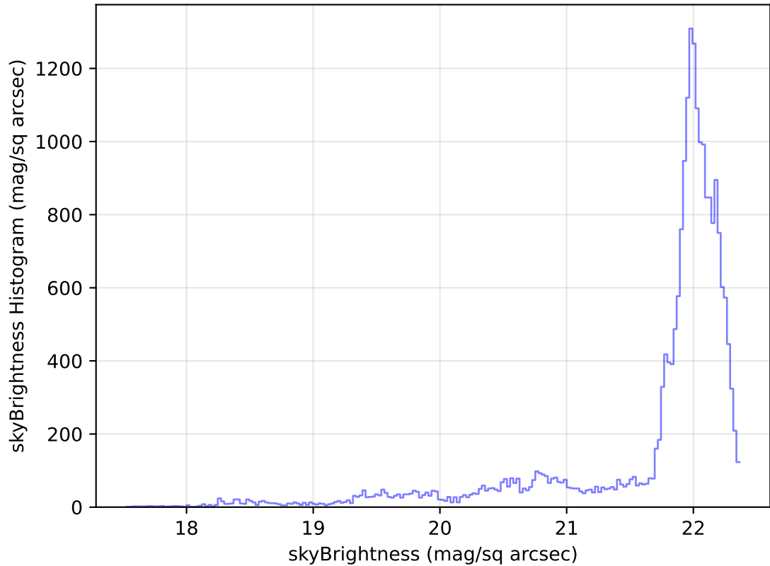
internal_u_expt45_nscale1.5v3.4_10yrs Yr 1 g band: skyBrightness Histogram
