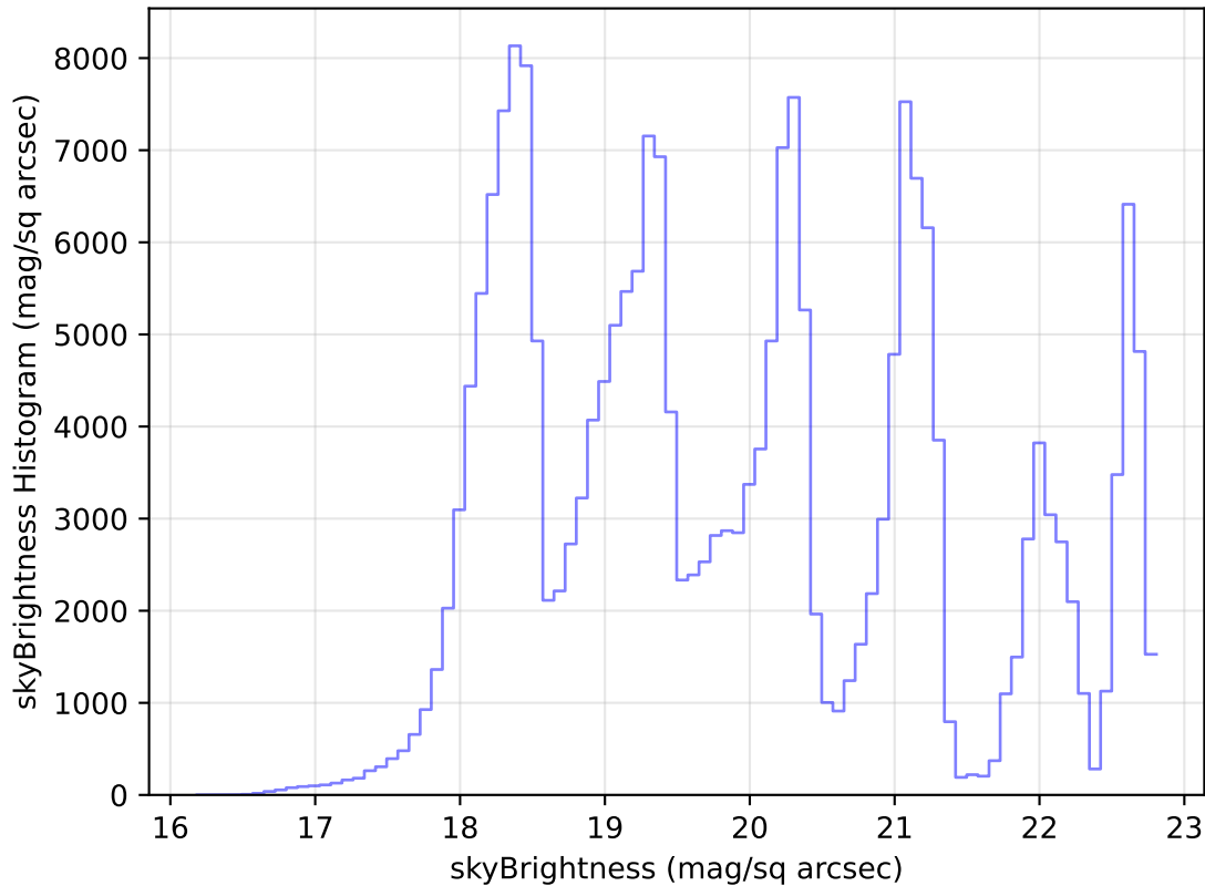
internal_u_expt45_nscale1.5v3.4_10yrs Yr 1 all bands: skyBrightness Histogram
