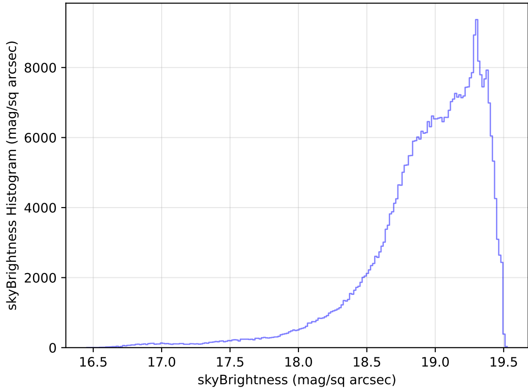
internal_u_expt45_nscale1.5v3.4_10yrs WFD z band: skyBrightness Histogram
