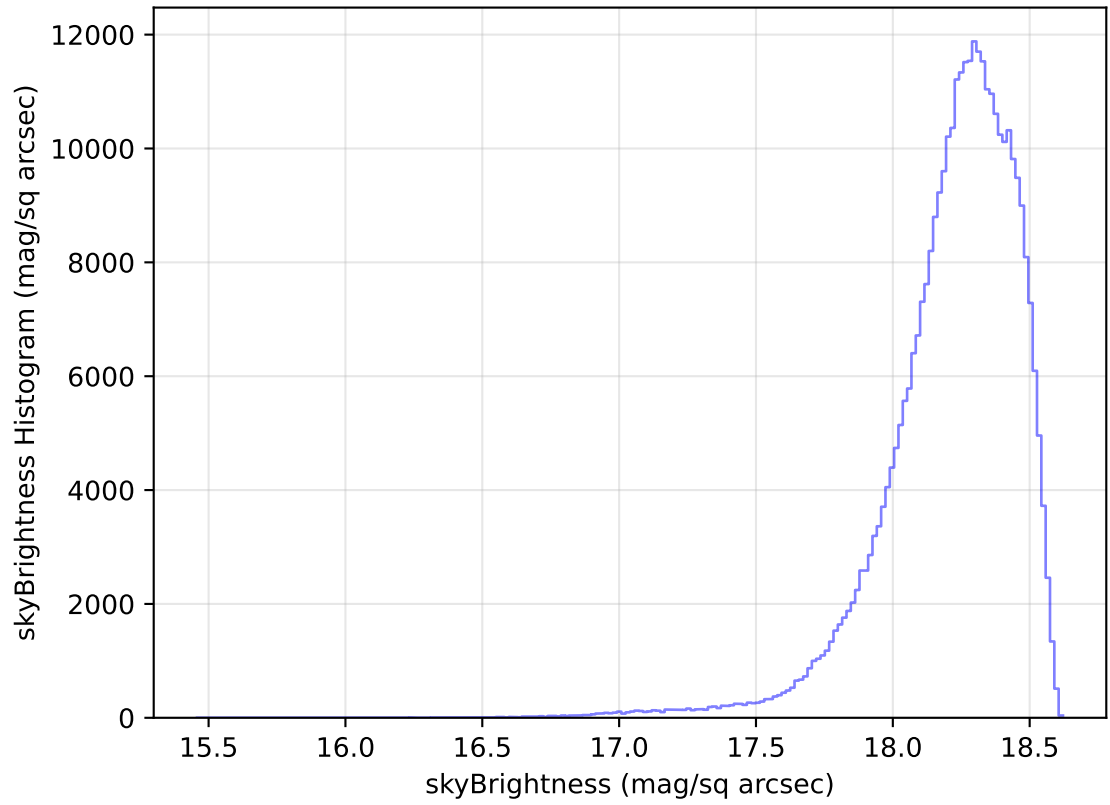
internal_u_expt45_nscale1.5v3.4_10yrs WFD y band: skyBrightness Histogram
