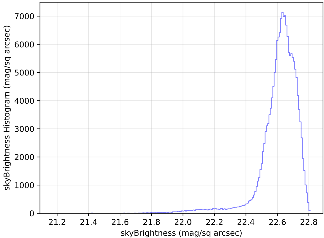
internal_u_expt45_nscale1.5v3.4_10yrs WFD u band: skyBrightness Histogram
